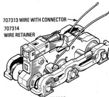
708300 Truck Assembly
