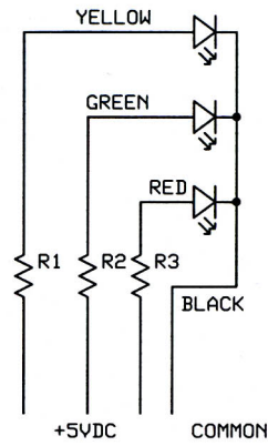
N SCALE SIGNAL
